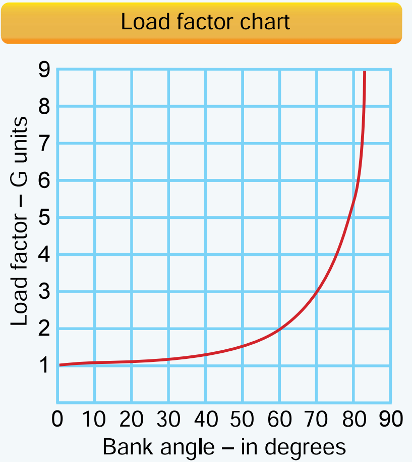
FIGURE 2.—Load Factor Chart.
